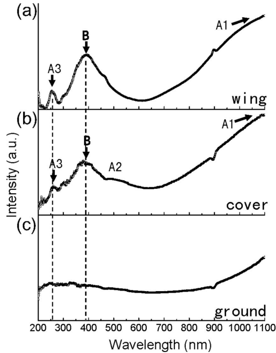
FIG. 4. Reflection spectra of the (a) original wing, (b) pure cover, and (c) pure ground scales with incidence angle as 33^\circ from the tail direction. The tiny peaks and bumps at 466 and 896 nm are from the measurement system.
