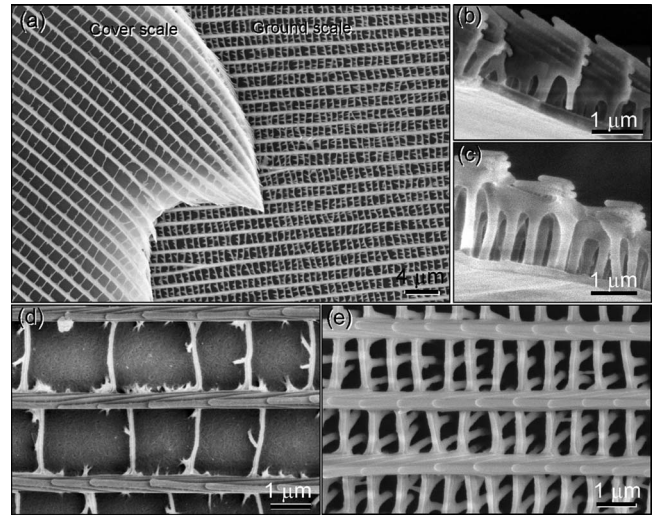
FIG. 2. (a) A low-magnification SEM image contains both the cover and ground scales. (b) and (c) are the cross-sectional SEM images; (d) and (e) are the plane-view SEM images of the cover and ground scales, respectively.
