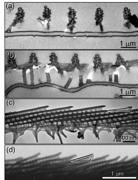
FIG. 3. Cross-sectional TEM images of the [(a) and (c)] cover and [(b) and (d)] ground scales viewing along and perpendicular to the ridges, respectively. The samples used for TEM imaging were coated with a thin layer of alumina by ALD. The inclination angles \alpha and \beta of the shelf to scale surface in cover and ground scales are close to 7^\circ and 17^\circ , respectively.
