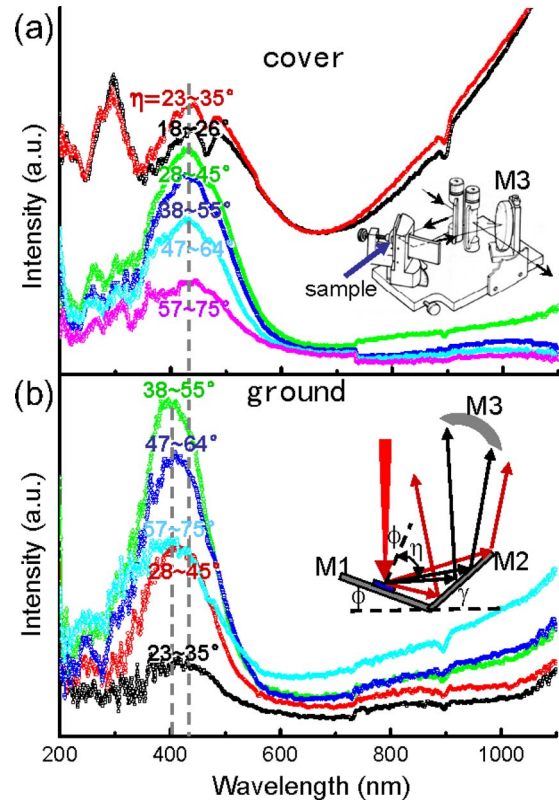
FIG. 5. (Color online) The reflection spectra measured from the (a) cover and (b) ground scales as a function of detector angle, with a fixed angle of 13^\circ for the incidence beam from the tail direction. The inset in (a) is the experimental setup. The inset in (b) is an in-plane optical diagram for the measurements.
